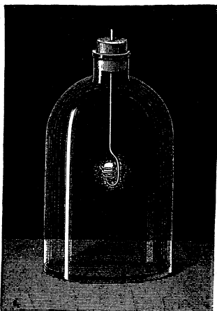
Fig. 33.—Combustion of the Diamond in Oxygen.
